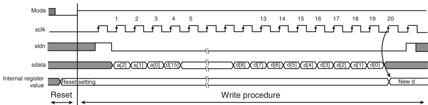
Figure 3-1. Write Chronogram
