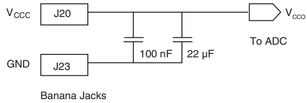
Figure 2-3. Power Supply Decoupling Scheme
