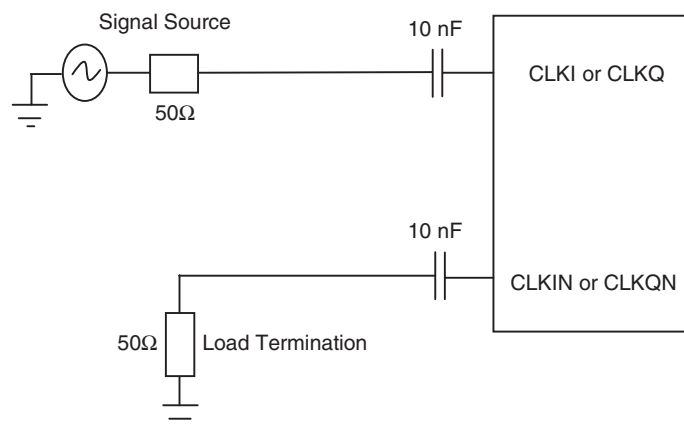
Figure 5-2. Clock Input Implementation
