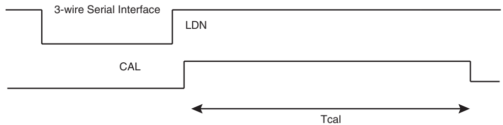
Figure 3-3. Internal Calibration Timing
